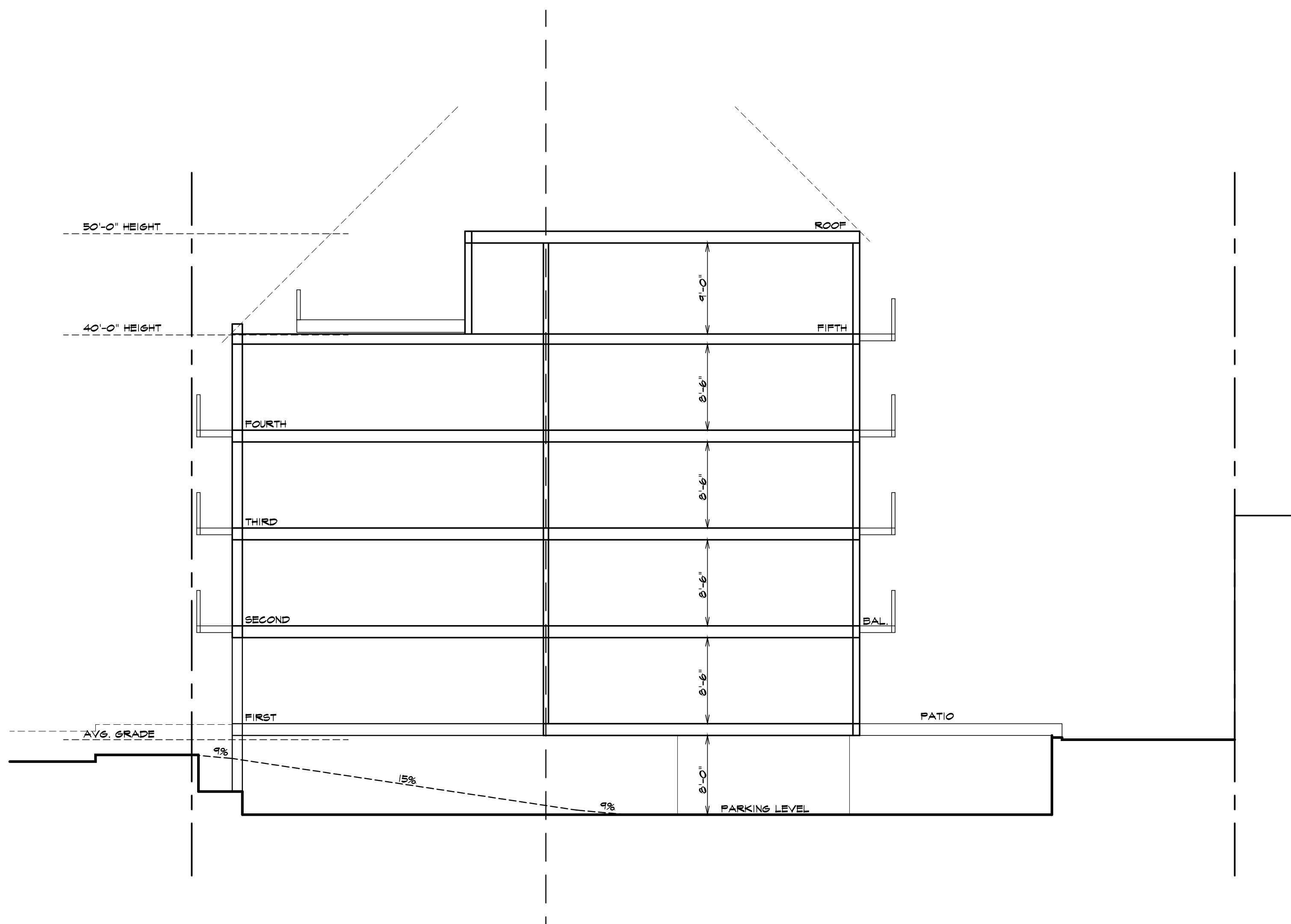
BUILDING SECTION 2341 ONTARIO RD. NW NEW BUILDING 1.26.2014
